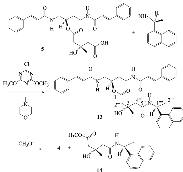
Scheme 2. Absolute stereochemistry determination of the HMGA moiety of pholiotic acid ( 5 ).
