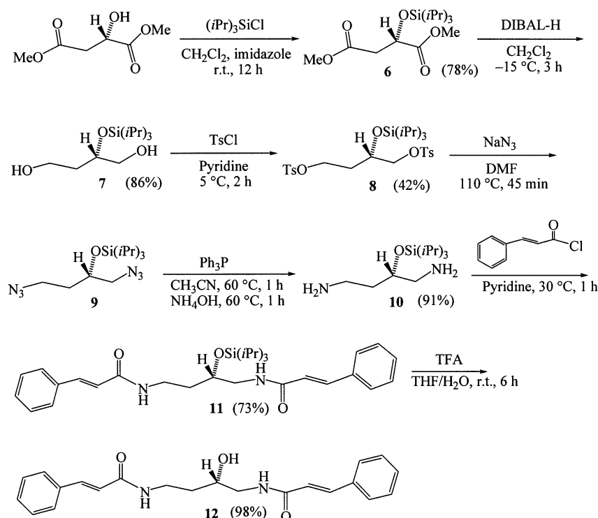
Scheme 1. Synthetic route to ( S )-2-hydroxyputrescine 1,4-dicinnamamide ( 12 ) from dimethyl ( S )-malate. Yields are in brackets.
